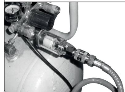
Fig. 6, filter connection (separator) Extol® Craft 8865101
